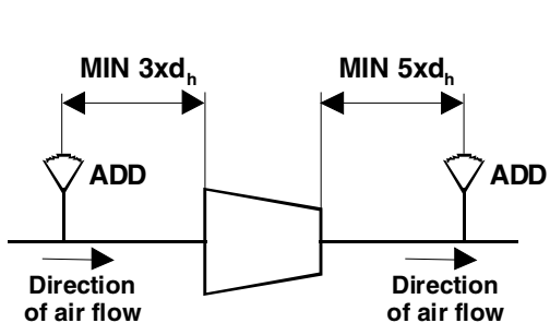
Fig. 10: Diameter decrease or increase in the air duct system
