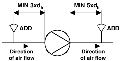
Fig. 4: Exhauster
